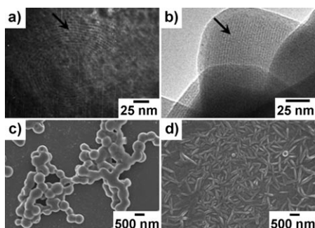
Figure 4. HRTEM images of a) spherical and b) fibrous assemblies. SEM images of SEOP-2 self-assemblies in different states after c) 30 min of UV irradiation; d) 30 min of visible-light irradiation following (c).
